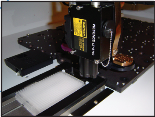
Microtiter plate Confocal Laser Measuring System
