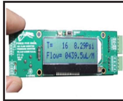
Microfluidics Flow and Pressure Monitor System
